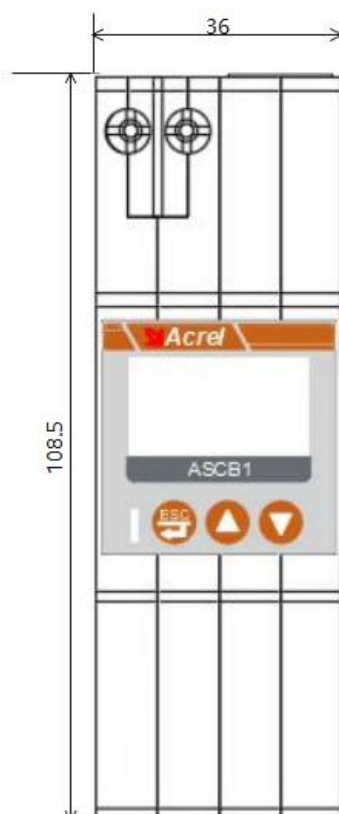
Figure 3 Dimension of intelligent gateway
